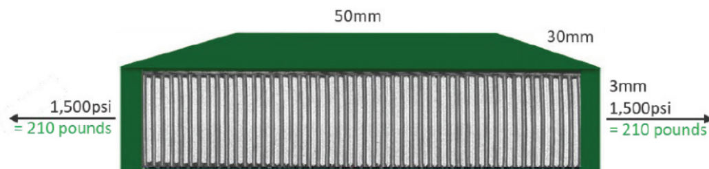
Silicon Swelling Forces in Enovix 3D Silicon™ Lithium-Ion Battery
