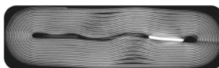
Conventional Li-Ion Battery (Jelly Roll) (1)
